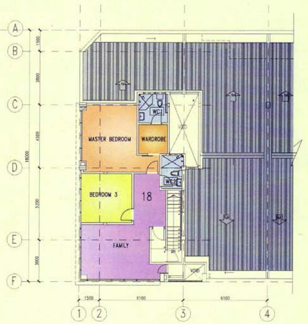
ROOF PLAN & THIRD FLOOR PLAN
