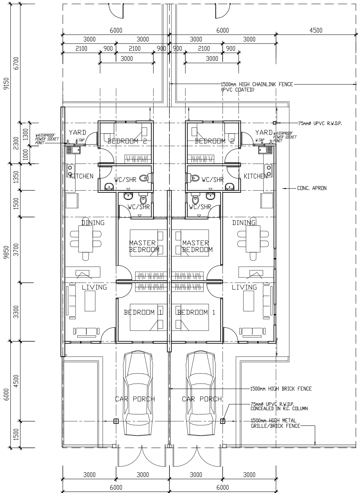
FLOOR LAYOUT PLAN (WALL-UP AREA= 66.30 sq.m/714 sq.ft) (REVISED DESIGN WITH 1-CAR CAR PORCH) SCALE: 1:100
